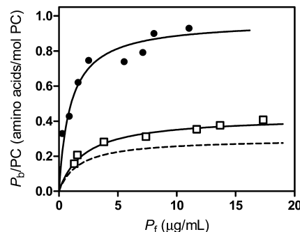
FIGURE 5: Binding isotherms of apoA-I V53C-pyrene (□) and F229C-pyrene (●). The solid lines are the theoretical binding isotherms calculated using eq 2 and the parameters shown in Table 2. The binding isotherm for WT apoA-I obtained from gel filtration experiments is also shown (dashed line) for comparison (ref 11).
