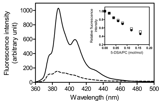
FIGURE 2: Fluorescence emission spectra of pyrene-labeled apoA-I V53C mutant in the lipid-free (dashed line) or bound to egg PC SUV (solid line). Protein and PC concentrations were 25 \mu g/mL and 1.0 mg/mL, respectively. The inset shows the relative changes in fluorescence of apoA-I V53C-pyrene ( \square ) and F229C-pyrene ( \bullet ) as a function of the molar ratio of 5-DSA to PC.
