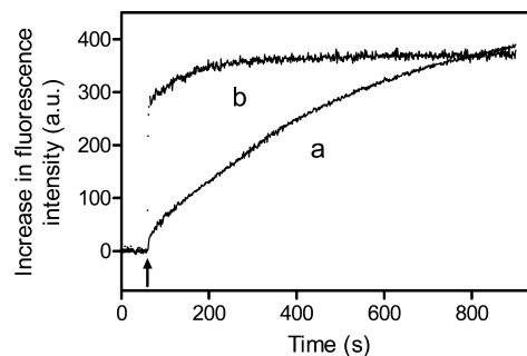
FIGURE 3: Time courses of increases in fluorescence intensity upon addition of egg PC SUV to apoA-I V53C-pyrene (trace a) and F229C-pyrene (trace b). SUV was added to apoA-I variants at final concentrations of 25 \mu g/mL protein and 1.0 mg/mL PC. Pyrene fluorescence was monitored at 385 nm with an excitation of 342 nm.
