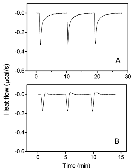
FIGURE 6: Isothermal titration curves for binding of WT apoA-I to egg PC SUV. (A) 8 \mu L aliquots of apoA-I solution (0.8 mg/mL) were injected into SUV (PC concentration of 15 mM). (B) 10 \mu L aliquots of SUV (PC concentration of 15 mM) were injected into apoA-I solution (0.3 mg/mL).
