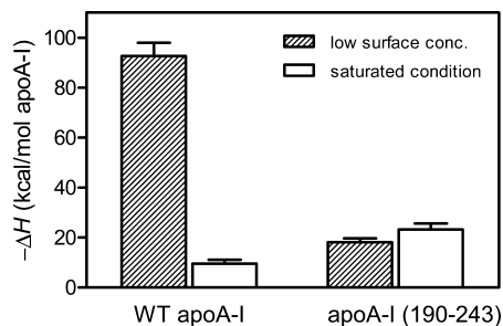
FIGURE 7: Binding enthalpies of apoA-I WT and 190–243 fragment to egg PC SUV obtained under two limiting conditions. Protein solutions were injected into excess SUV at a PC-to-protein molar ratio of >10,000 (low surface concentration), or SUV was injected into excess protein at a PC-to-protein molar ratio of <10 (saturated condition).
