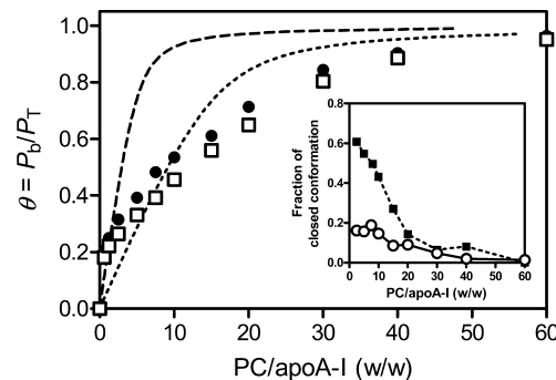
FIGURE 8: Increase in fluorescence intensity of apoA-I V53C-pyrene ( \square ) and F229C-pyrene ( \bullet ) upon binding to egg PC/cholesterol (17/3 mol/mol) SUV. Protein concentration was 25 \mu g/mL. The titration curves for binding of V53C-pyrene (dotted line) and F229C-pyrene (dashed line) to egg PC SUV are also shown for comparison. The inset shows the effect of cholesterol on the change in the fraction of closed conformation of the helix bundle in apoA-I bound to SUV. \blacksquare , egg PC SUV; \circ , egg PC/cholesterol (17/3) SUV.
