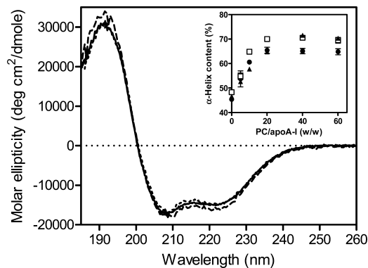
FIGURE 1: Far-UV CD spectra of WT (solid line), V53C-pyrene (dashed line), and F229C-pyrene (dotted line) apoA-I in the lipid-free state. The inset shows the increase in \alpha -helix content of the apoA-I variants bound to egg PC SUV as a function of the weight ratio of PC to apoA-I. \blacktriangle , WT apoA-I; \square , apoA-I V53C-pyrene; \bullet , apoA-I F229C-pyrene. Protein concentration was 50 \mu g/mL.
