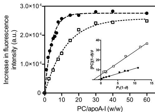
FIGURE 4: Increase in fluorescence intensity of apoA-I V53C-pyrene (□) and F229C-pyrene (●) as a function of the weight ratio of PC to apoA-I. Protein concentration was 25 \mu\text{g}/\text{mL} . The inset shows the linearized plots using eq 4.
