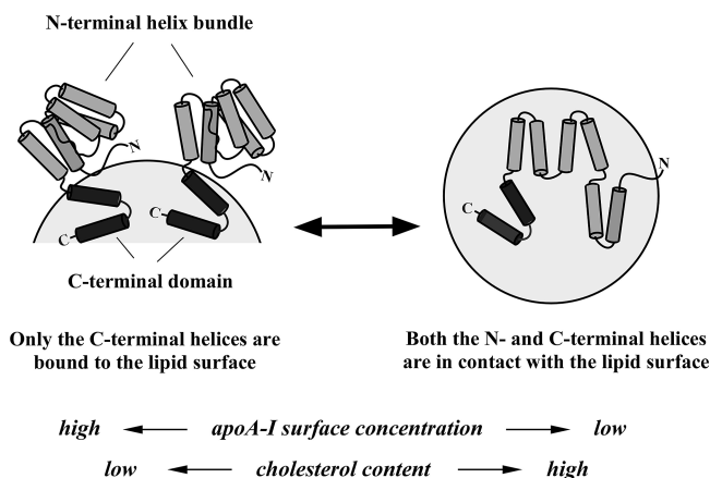
FIGURE 9: Model of two possible conformations of apoA-I at the surface of a spherical lipid particle. At high apoA-I surface concentration, the N-terminal helix bundle remains closed and out of contact with the lipid surface (left). At low surface coverage where a greater surface area is available, the helix bundle is open so that the \alpha -helices can make contact with the lipid surface (right). Cholesterol content in the lipid surface also modulates the equilibrium between the two conformations.
